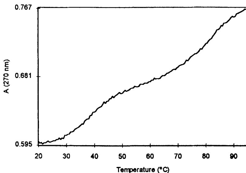
FIGURE 3 : Absorbance vs temperature plot for the h_{26}.s_{11} - m^5CBr^5U triplex (see table 2) in 1M NaCl, 100 mM sodium phosphate / citric acid buffer at pH 6.5.
