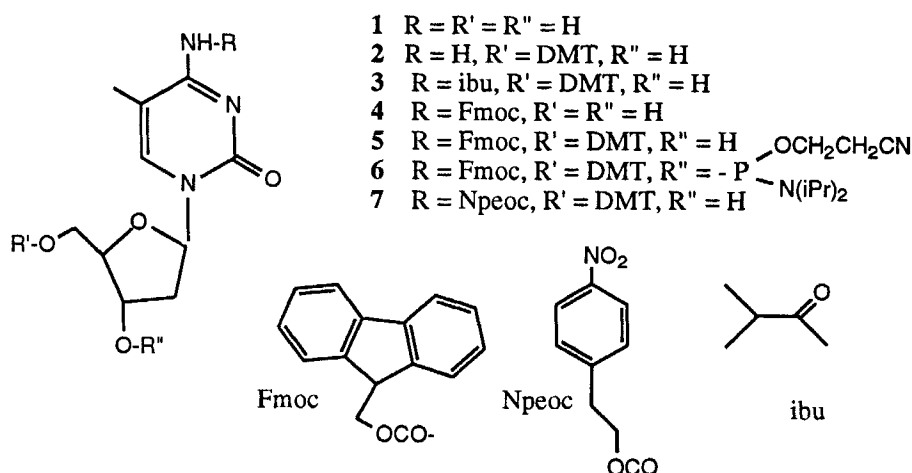
FIGURE 2: 5-Methyl-2'-deoxycytidine derivatives prepared in this work.
