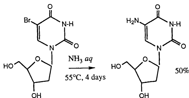
FIGURE 1: Conversion of 5-bromo-2'-deoxyuridine to 5-amino-2'-deoxyuridine in aqueous ammonia solutions .
